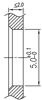
Panel cut-out
